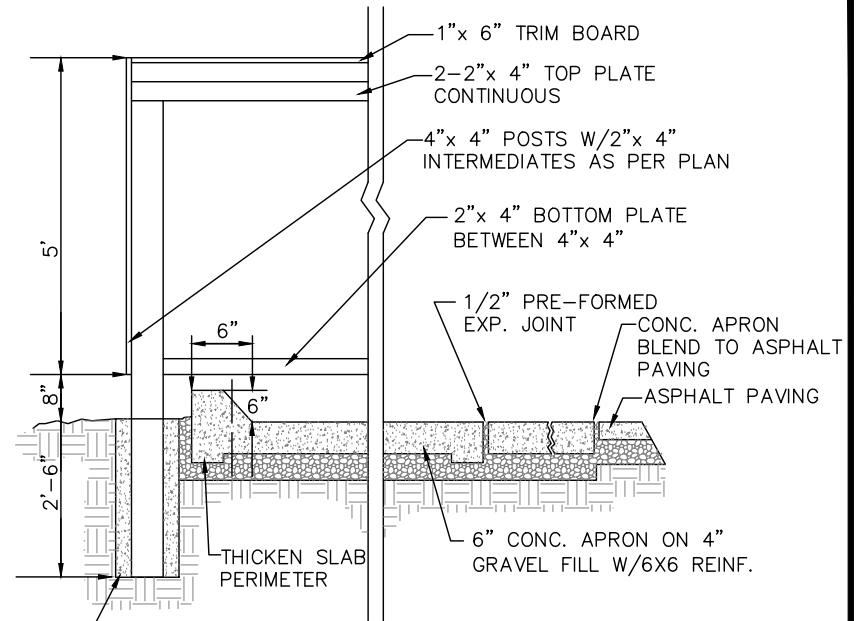
"A-A" "B-B" SECTION TRASH ENCLOSURE
