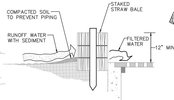
BALE INLET FILTER
