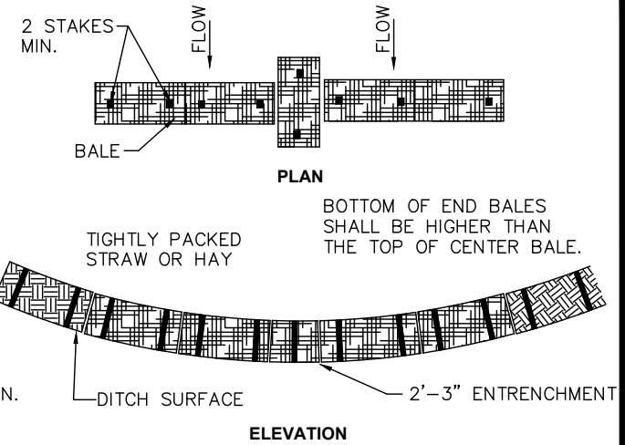
BALE DITCH CHECK
